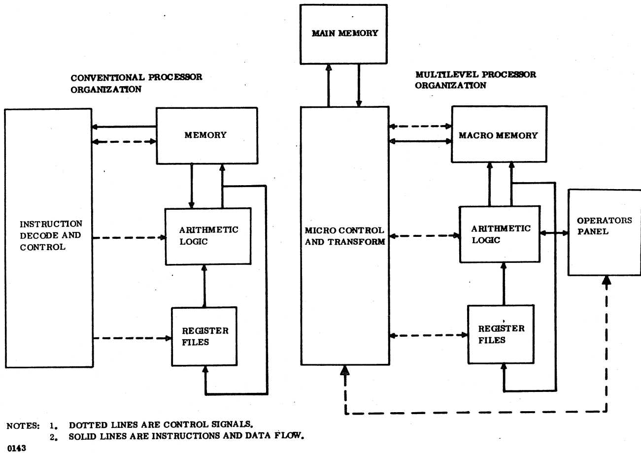
Figure 1-1. Digital Processor Organizations
