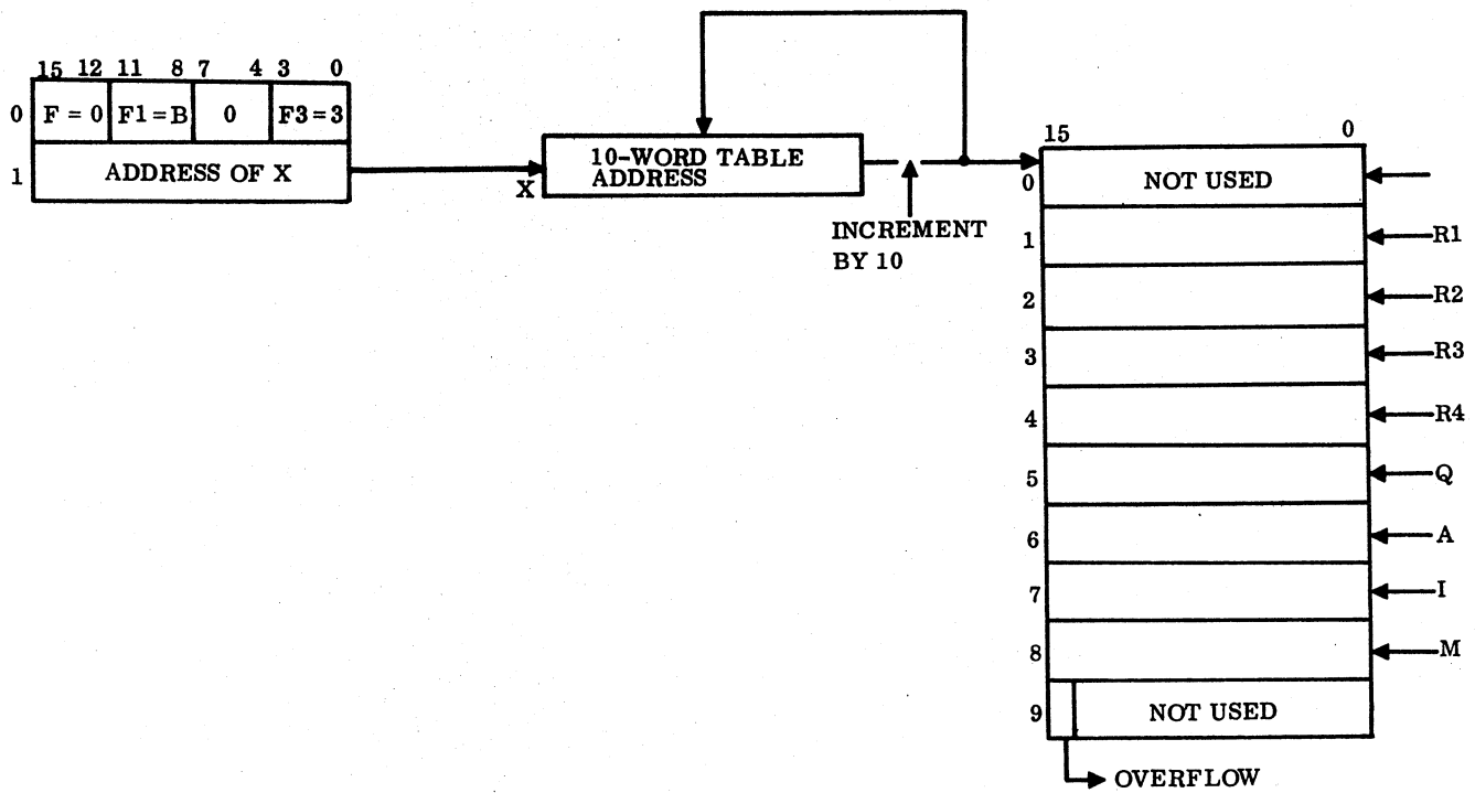
Figure 4-2. SRG Instruction
