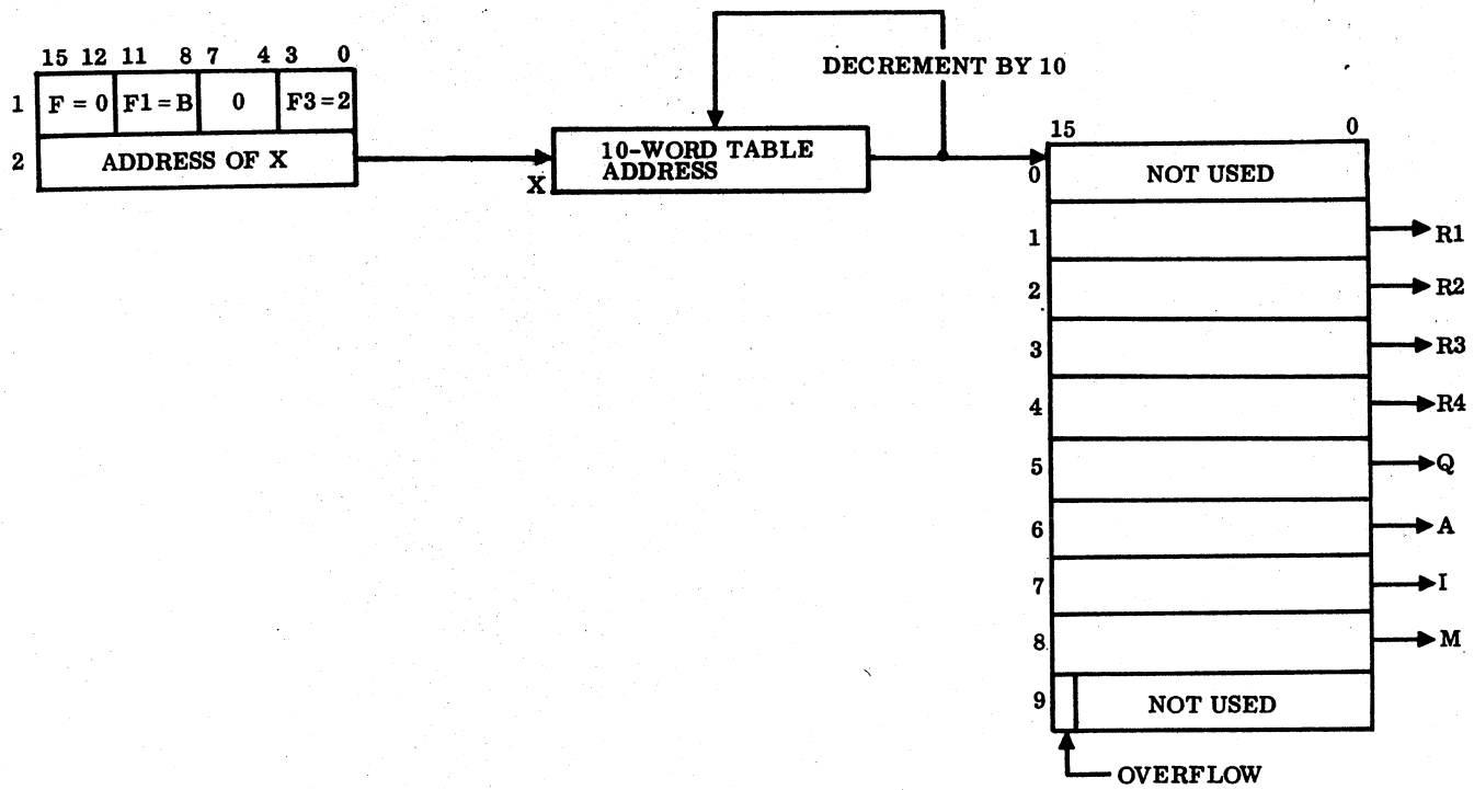
Figure 4-1. LRG Instruction
