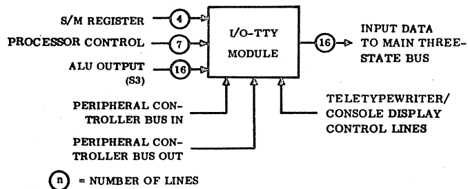
Figure 2-4. Major I/O-TTY Signal Flow Paths
